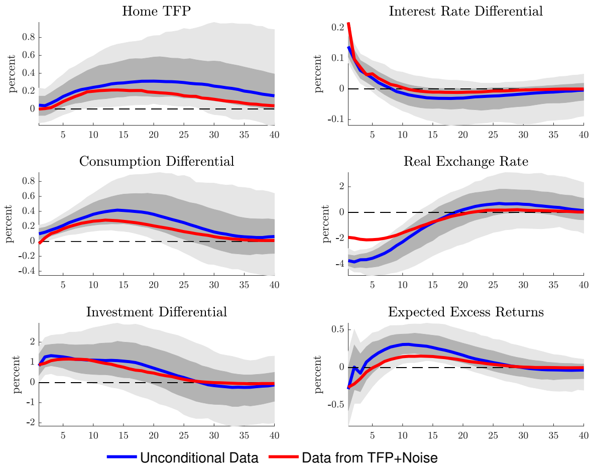
Figure 12: Chahrouh and Jurado (2021) vs Uhlig (2003)
